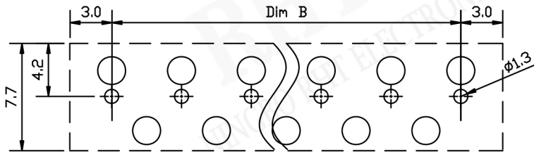
PCB LAYOUT
