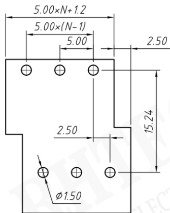
PCB LAYOUT
