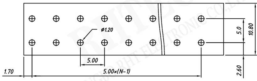
PCB LAYOUT
