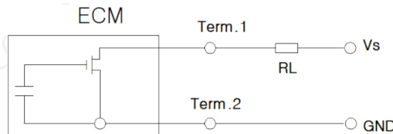
Schematic diagram VS=2V RL=2.2K
