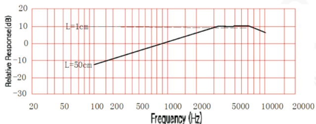
Frequency response
