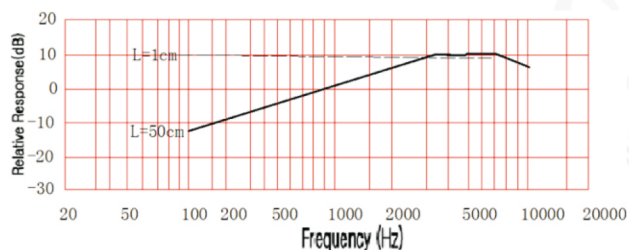
Frequency response
