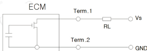
Schematic diagram VS=2V RL=2.2K
