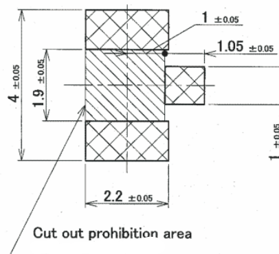
RECOMMENDED FOOTPRINT PATTERN
