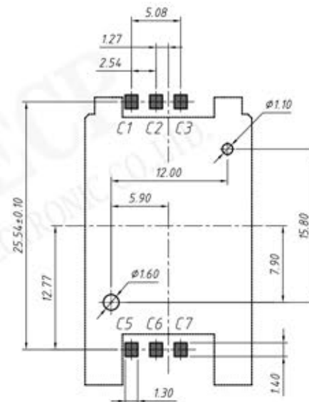
Reference PCB layout Unit:mm tolerance:±0.05
