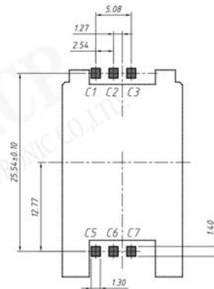
Reference PCB layout Unit:mm tolerance:±0.05
