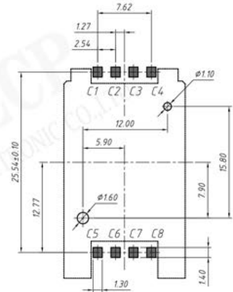
Reference PCB layout Unit:mm tolerance:±0.05
