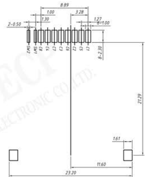
RECOMMENDED PCB LAYOUT GENERAL TOLERANCE ±0.05
