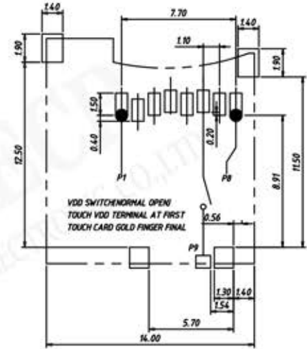
RECOMMENDED PCB LAYOUT GENERAL TOLERANCE ±0.05
