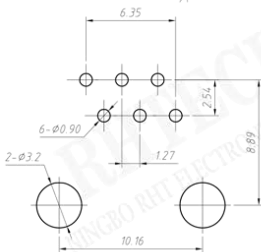
PCB Layout
