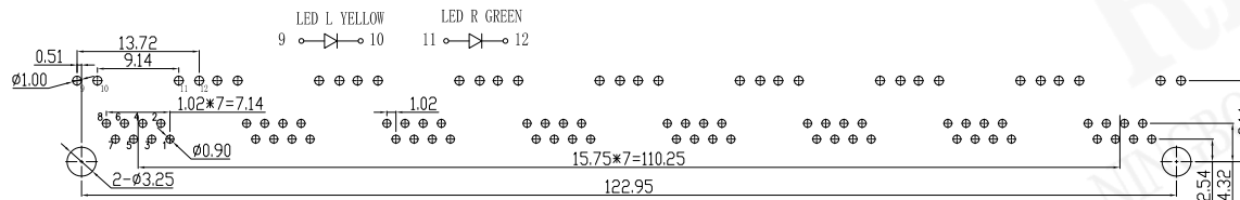
PC Board Layout
